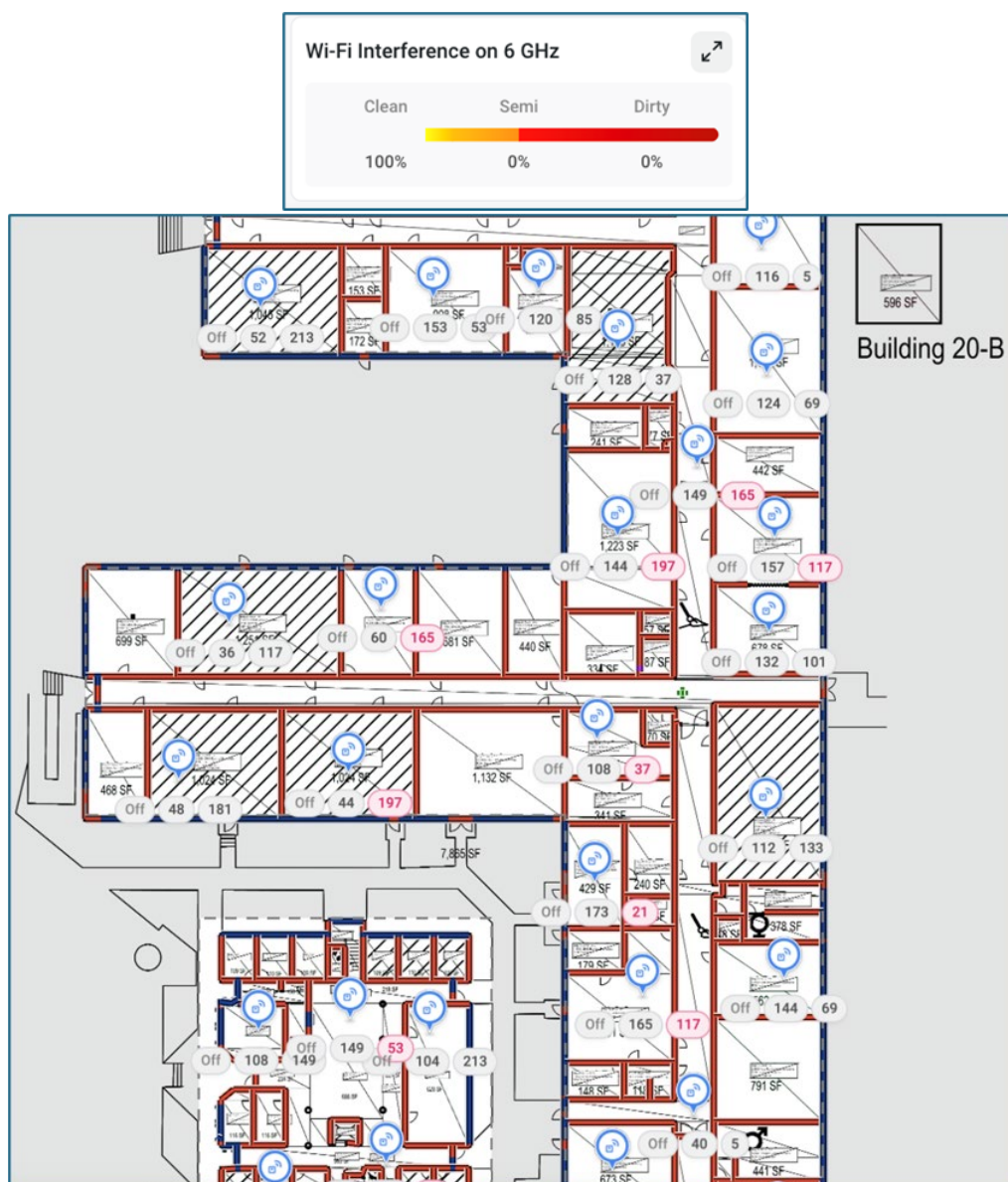
Figure 3: University Building Wi-Fi Interference (Fourteen 80 MHz Channels, full 6 GHz Band)
